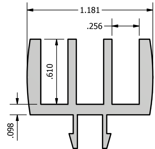
22.1075/1 GUIDE PROFILE 2 CROSS SECTION
